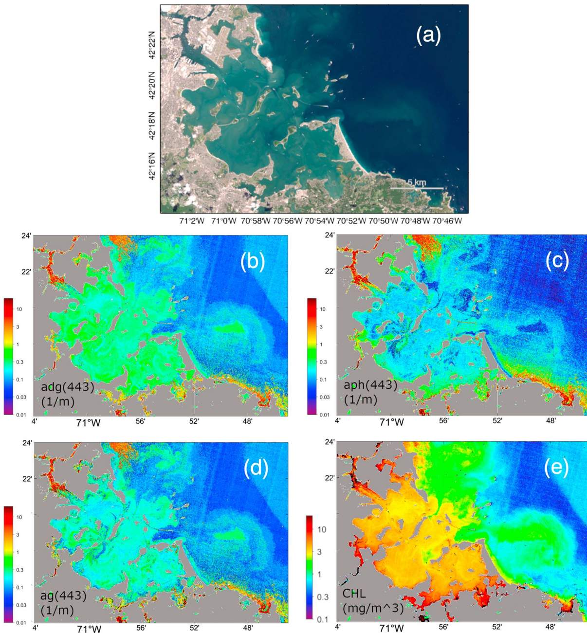
Figure 8. Landsat 8/Operational Land Imager true color image (LC80120312015240) of Boston Harbor and Massachusetts Bay (panel a) and mapping products of retrieved component absorption coefficients a_{ph}(443) , a_{dg}(443) , and a_g(443) (unit: per meter) from Semi-Analytical algorithm with a Virtual-band Estimator (panels b–d). Panel (e) is the chlorophyll a concentrations (unit: milligram per cubic meter) derived from the fourth-order polynomial function of R_{rs}(482)/R_{rs}(561) ratios with coefficients determined by NASA.
