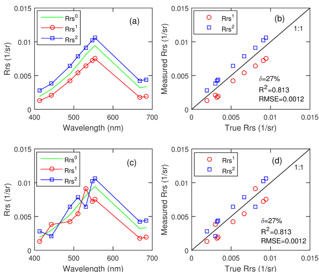
Figure 12. Application and limitation of scatter-plot practice in evaluating the data quality of R_{rs} spectra. The R_{rs}^0 spectrum (in green) represents true values. The R_{rs}^1 and R_{rs}^2 spectra refer to two example measurements. The scatter-plot of Figure 12b represents the measurement scenario in Figure 12a, where the R_{rs}^1 and R_{rs}^2 spectra retain the same shapes as R_{rs}^0 . Figure 12c represents another situation when the R_{rs}^1 and R_{rs}^2 spectra are erroneously measured (for brevity, we simply switched R_{rs} values at some bands between R_{rs}^1 and R_{rs}^2 spectra). Interestingly, the resulted new scatter-plot in Figure 12d is exactly the same with Figure 12b, with the same error statistics.
