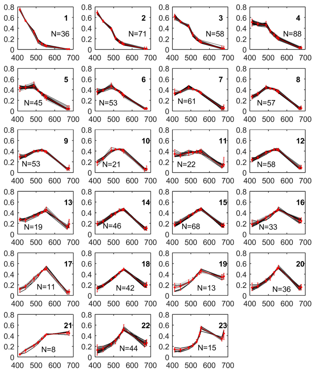
Figure 3. Clustering of 23 optical water types. The gray-black curves represent the normalized R_{rs} spectra classified into each water type. The mean R_{rs} spectra are highlighted in red, with the error bars characterizing the maximum and minimum values. And in each water type, the total numbers of available R_{rs} spectra are also given.
