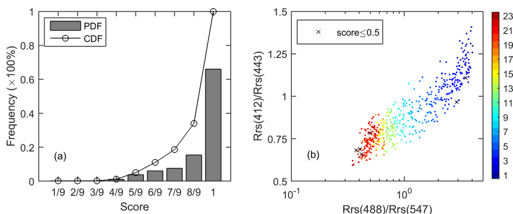
Figure 5. (a) Frequency distribution of the scores assigned to the simulated R_{rs} data. The scores are given in fractional numbers with the numerators referring to the numbers of good-quality wavebands. (b) Ratio distribution of R_{rs}(412)/R_{rs}(443) against R_{rs}(488)/R_{rs}(547) . The corresponding 23 water types are denoted in colors and the spectra identified with low QA scores ( \leq 0.5 ) are denoted with cross symbols in black.
