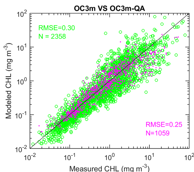
Figure 11. Comparison of estimated [CHL] with in situ measured [CHL]. The original (not quality controlled) data are compared to OC3m modeled data (in green open circles). The quality controlled data (in pink dots, with the highest scores) are compared to OC3m-QA estimated data. OC3m-QA has new model coefficients developed from these highest-score data ( N = 1059 , excluding those from the Arctic and Southern Oceans) only. The OC3m-QA has the new model coefficients as 0.2053, -2.0159 , 1.1159 , -1.3885 , and 0.5474 .
