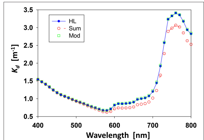
FIGURE 1 | Comparison of K_d spectra between Hydrolight simulation (blue), sum of individual components (red), and that from semi-analytical model based on bulk IOPs (green). The range for K_d is between surface and 5 m.
