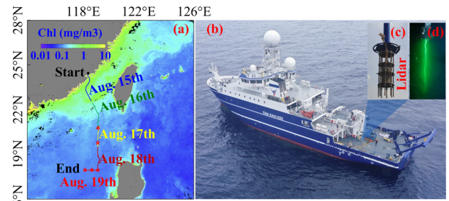
Fig. 4. (a) R/V navigation trajectory with lidar, overlaid on a monthly averaged Chl-a map from ocean color satellite. Red pentagon stars indicate R/V operation station positions. (b) Lidar installation on the R/V. (c) Installation process illustration. (d) Underwater operation of the lidar. Chl-a data sourced from NASA MODIS standard monthly composite for August 2023.
